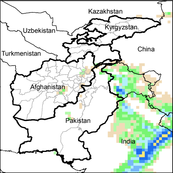
Daily Precip. Forecast for 16 Dec., 2014
