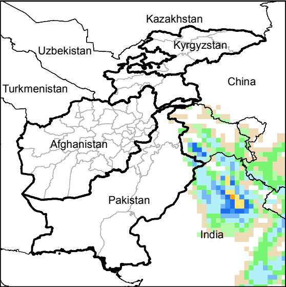
Daily Precip. Forecast for 17 Dec., 2014
