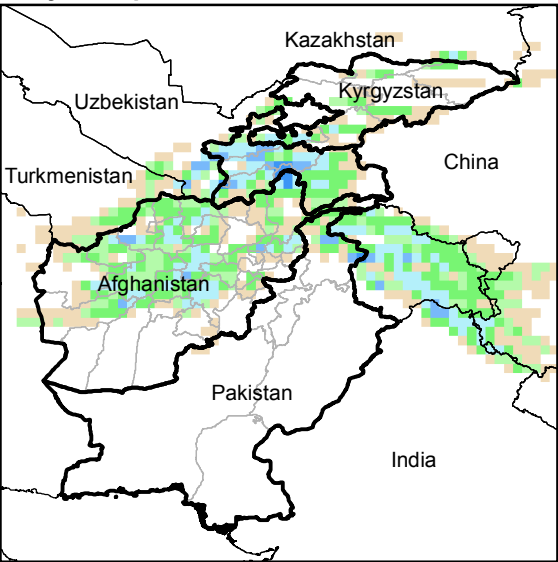
Daily Precip. Forecast for 25 Dec., 2014
