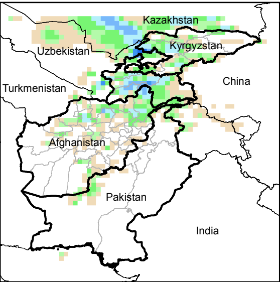
Daily Precip. Forecast for 28 Dec., 2014
