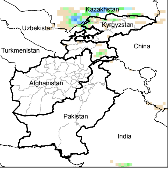
Daily Precip. Forecast for 2 Jan., 2015
