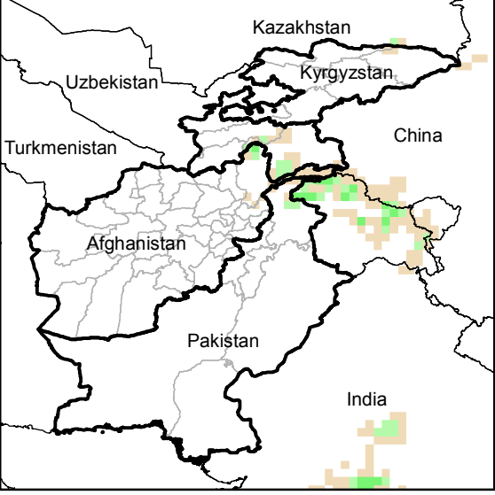
Daily Precip. Forecast for 31 Dec., 2014
