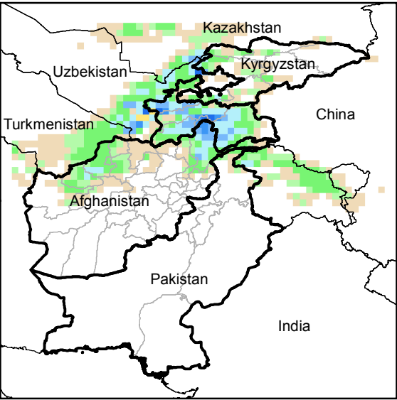
Daily Precip. Forecast for 5 Jan., 2015
