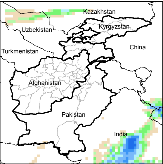
Daily Precip. Forecast for 4 Jan., 2015
