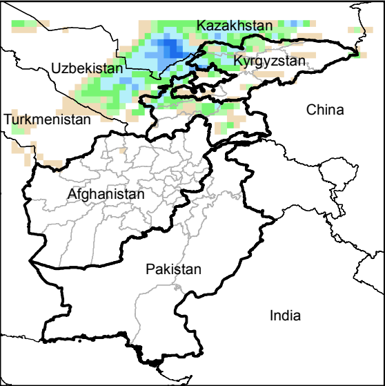
Daily Precip. Forecast for 12 Jan., 2015
