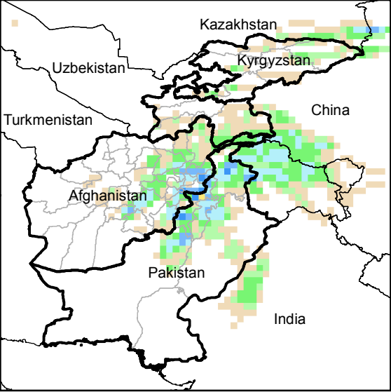
Daily Precip. Forecast for 13 Jan., 2015
