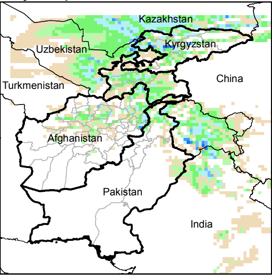
Daily Precip. Forecast for 23 Jan., 2015
