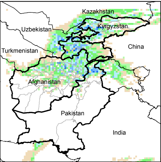
Daily Precip. Forecast for 27 Jan., 2015
