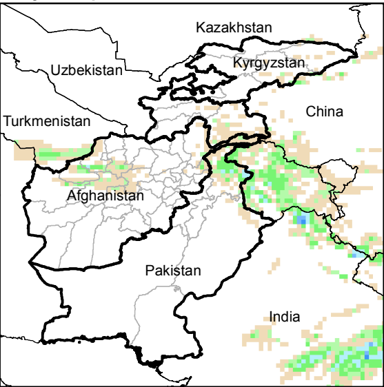
Daily Precip. Forecast for 30 Jan., 2015
