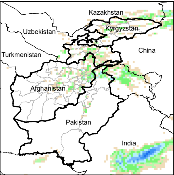
Daily Precip. Forecast for 28 Jan., 2015
