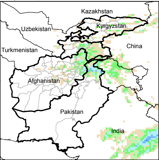
Daily Precip. Forecast for 29 Jan., 2015
