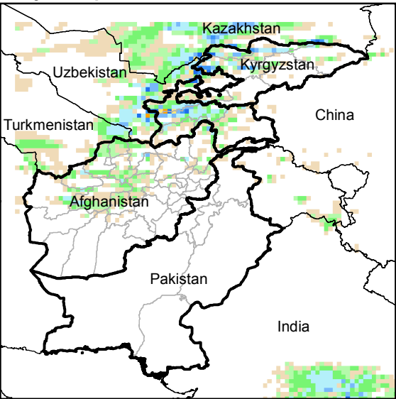
Daily Precip. Forecast for 14 Feb., 2015
