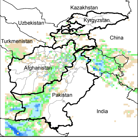
Daily Precip. Forecast for 27 Feb., 2015
