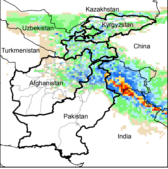
Daily Precip. Forecast for 25 Feb., 2015
