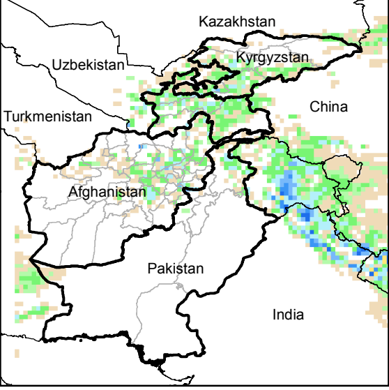
Daily Precip. Forecast for 26 Feb., 2015
