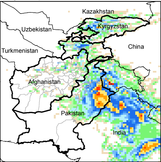
Daily Precip. Forecast for 18 Mar., 2015
