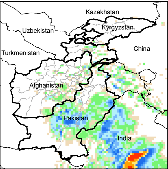
Daily Precip. Forecast for 17 Mar., 2015
