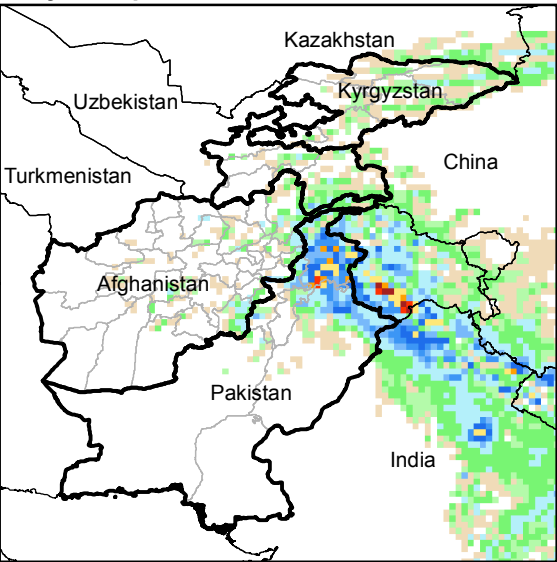
Daily Precip. Forecast for 19 Mar., 2015
