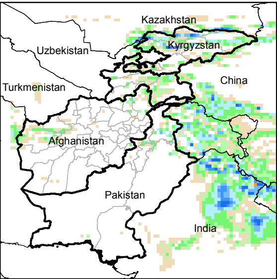
Daily Precip. Forecast for 7 Apr., 2015
