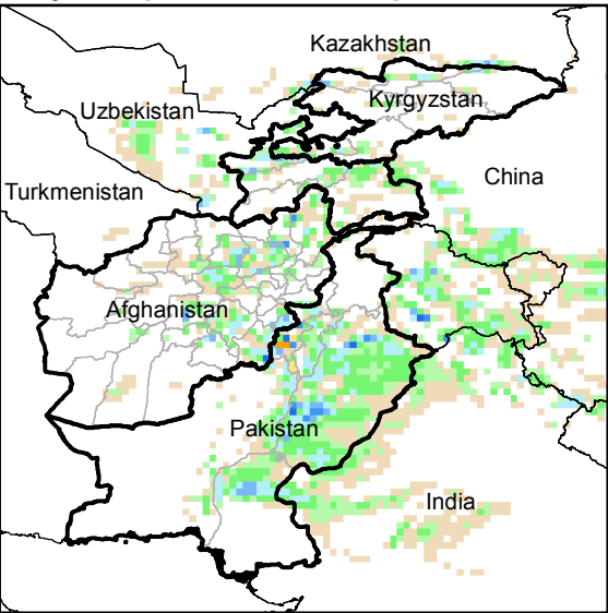
Daily Precip. Forecast for 9 Apr., 2015
