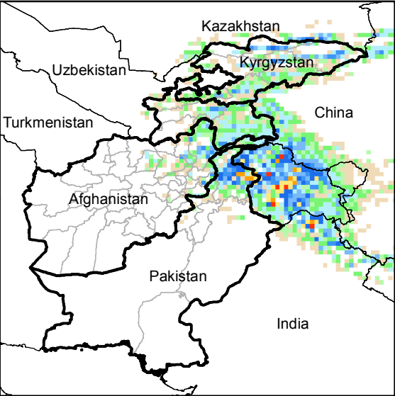
Daily Precip. Forecast for 20 Apr., 2015
