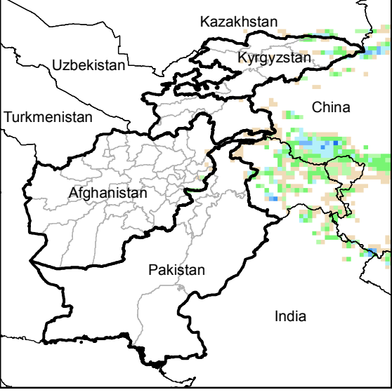
Daily Precip. Forecast for 21 Apr., 2015
