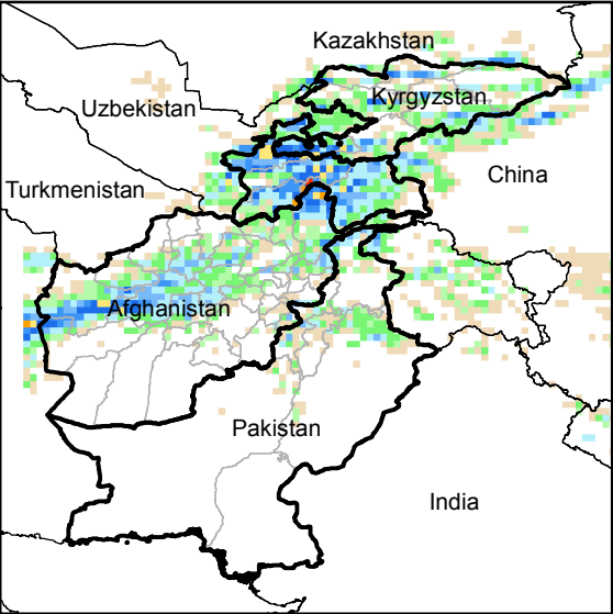
Daily Precip. Forecast for 18 Apr., 2015
