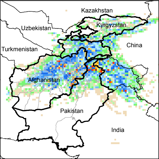
Daily Precip. Forecast for 19 Apr., 2015
