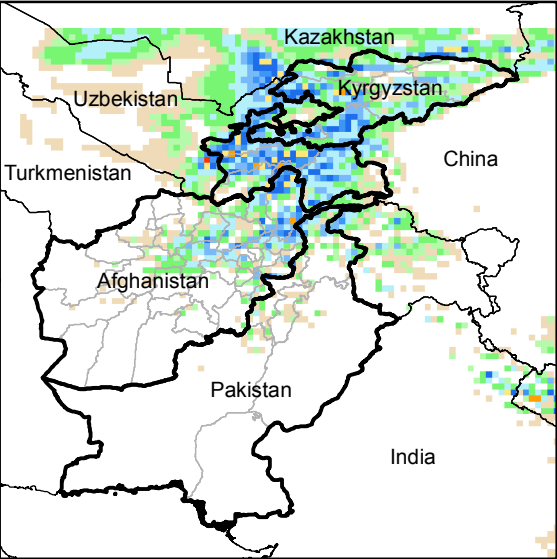
Daily Precip. Forecast for 26 Apr., 2015
