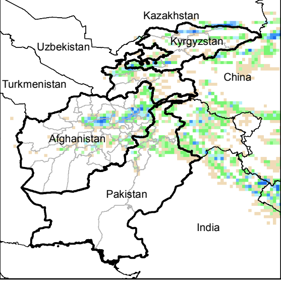
Daily Precip. Forecast for 29 Apr., 2015
