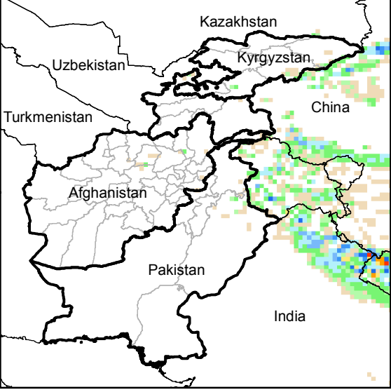
Daily Precip. Forecast for 28 Apr., 2015
