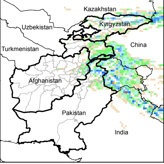
Daily Precip. Forecast for 27 Apr., 2015
