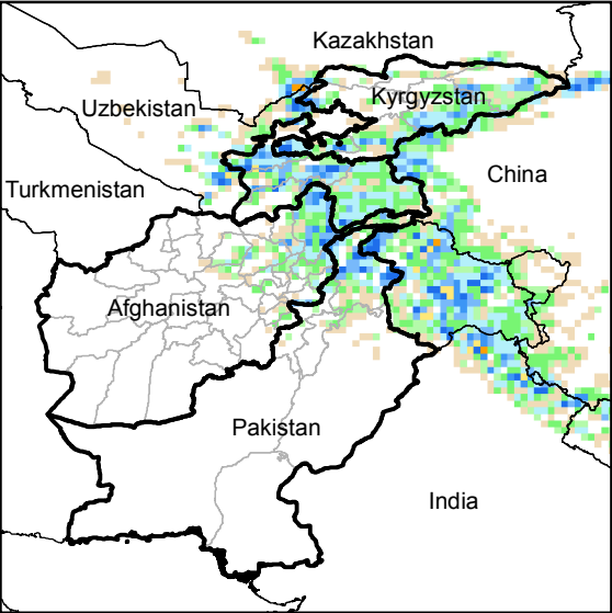
Daily Precip. Forecast for 3 May., 2015
