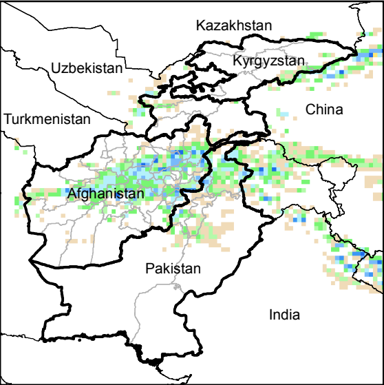
Daily Precip. Forecast for 2 May., 2015
