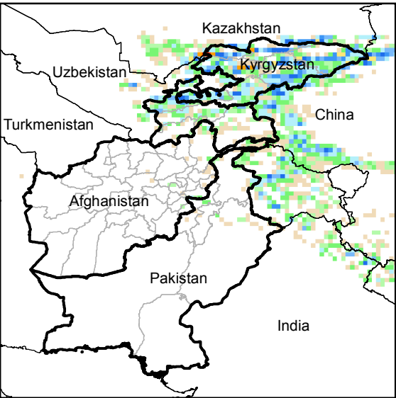
Daily Precip. Forecast for 4 May., 2015
