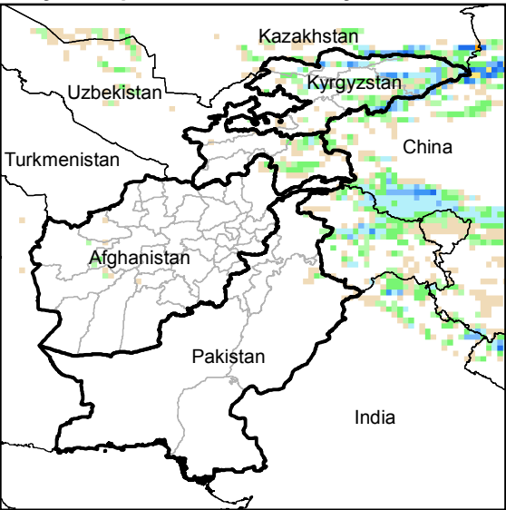
Daily Precip. Forecast for 5 May., 2015
