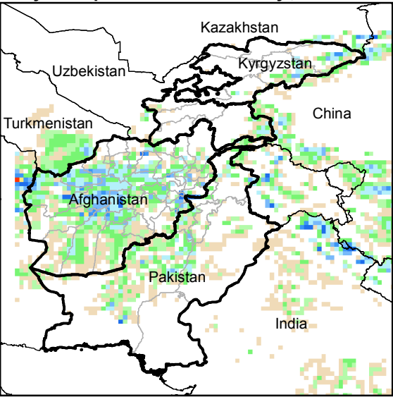
Daily Precip. Forecast for 10 May., 2015
