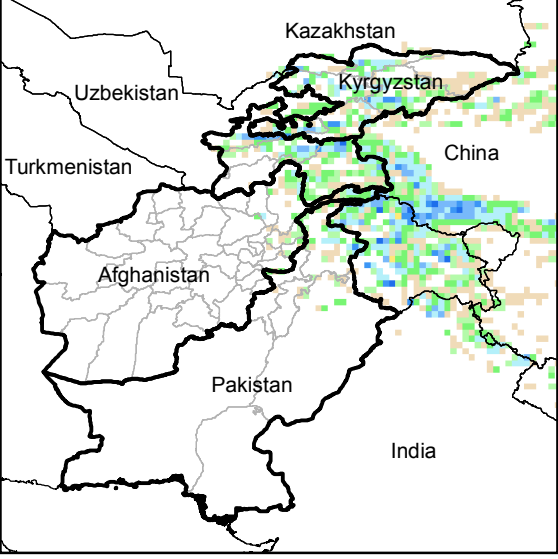
Daily Precip. Forecast for 30 May., 2015
