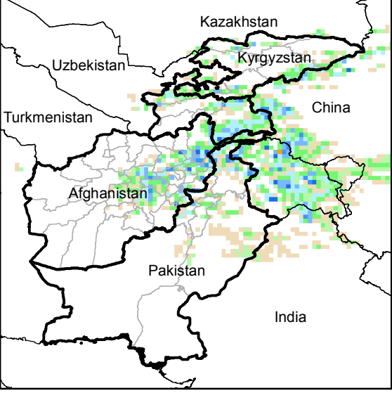
Daily Precip. Forecast for 29 May., 2015
