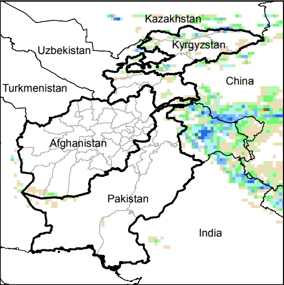
Daily Precip. Forecast for 26 May., 2015
