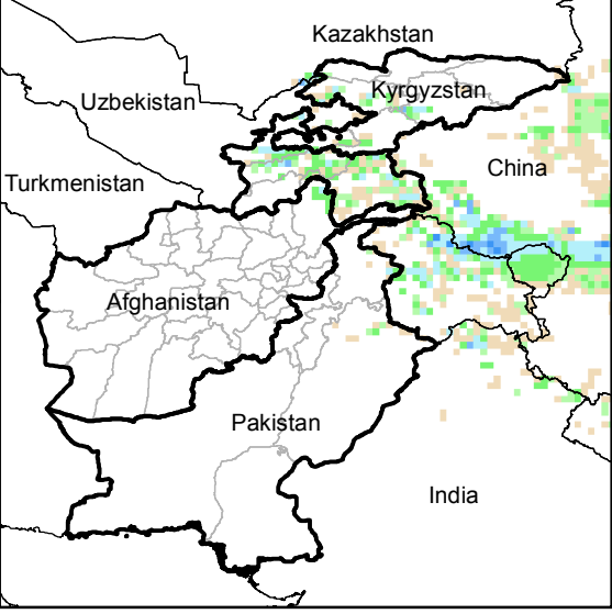
Daily Precip. Forecast for 31 May., 2015
