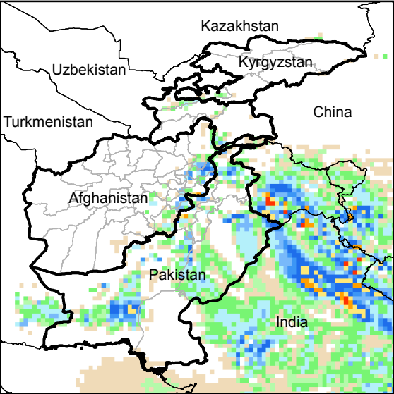
Daily Precip. Forecast for 15 Jul., 2015
