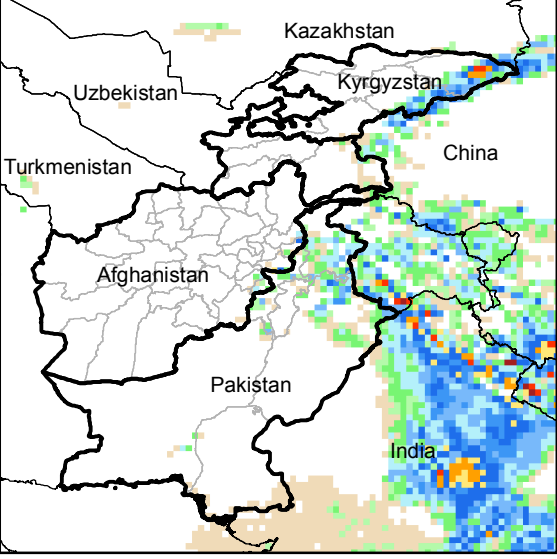
Daily Precip. Forecast for 7 Aug., 2015
