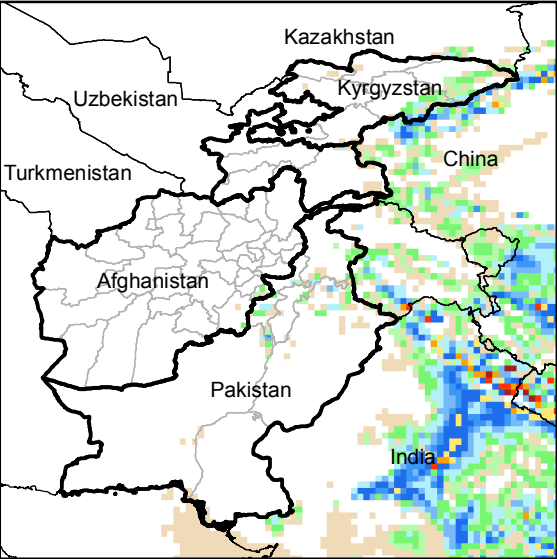
Daily Precip. Forecast for 9 Aug., 2015
