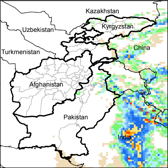
Daily Precip. Forecast for 8 Aug., 2015
