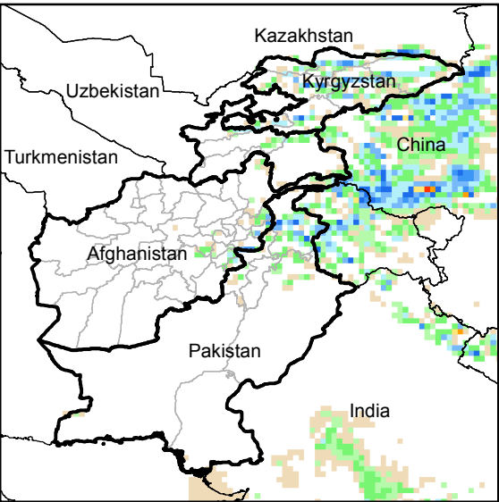
Daily Precip. Forecast for 9 Sep., 2015
