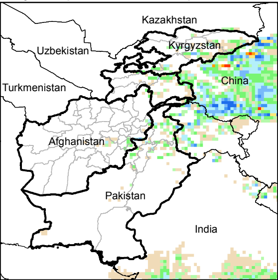
Daily Precip. Forecast for 10 Sep., 2015
