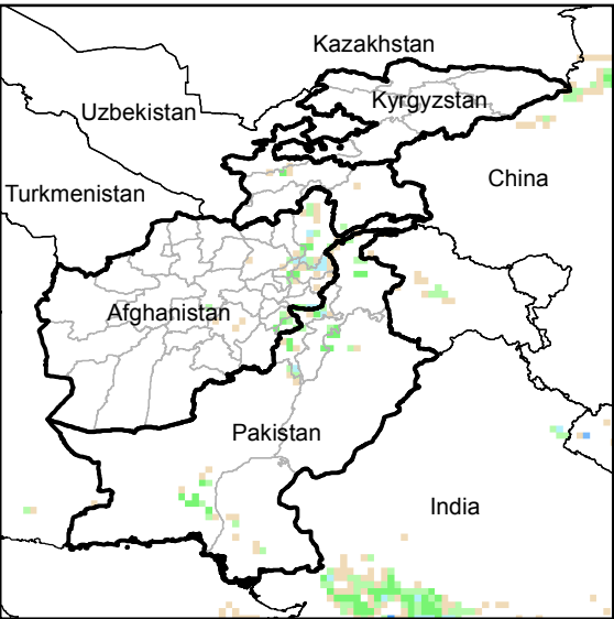
Daily Precip. Forecast for 12 Sep., 2015
