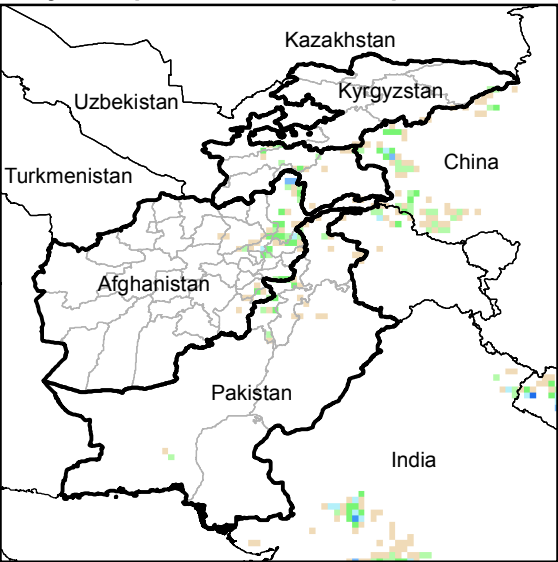
Daily Precip. Forecast for 13 Sep., 2015
