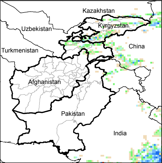
Daily Precip. Forecast for 14 Sep., 2015
