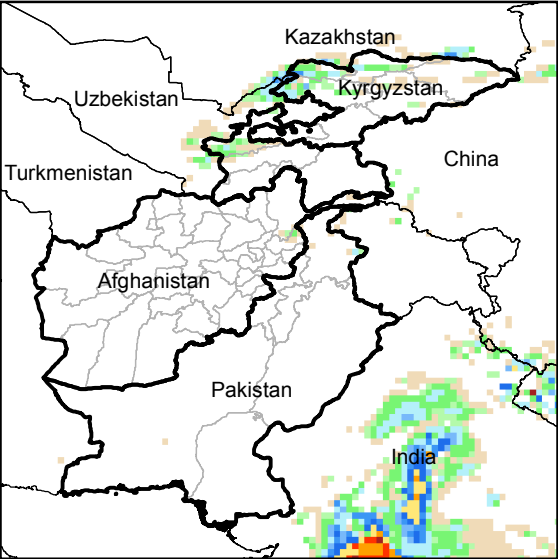
Daily Precip. Forecast for 18 Sep., 2015
