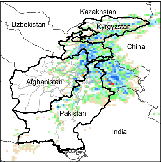
Daily Precip. Forecast for 22 Oct., 2015
