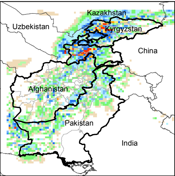
Daily Precip. Forecast for 21 Oct., 2015
