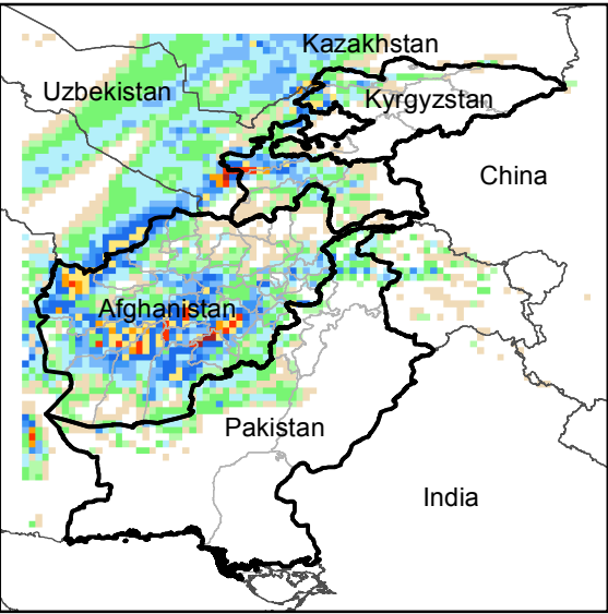
Daily Precip. Forecast for 11 Nov., 2015
