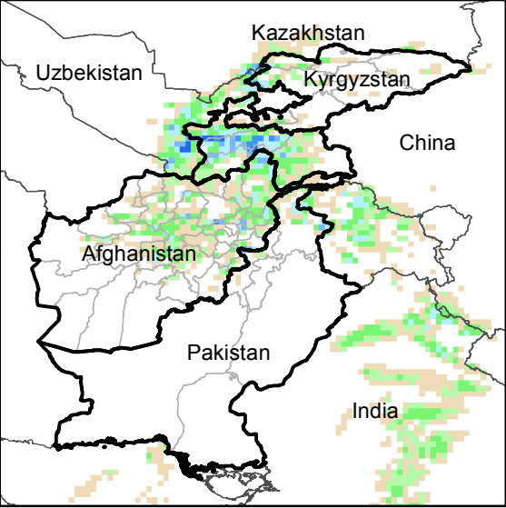
Daily Precip. Forecast for 7 Jan., 2016
