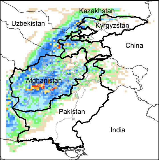
Daily Precip. Forecast for 6 Jan., 2016
