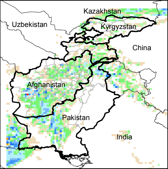
Daily Precip. Forecast for 2 Mar., 2016
