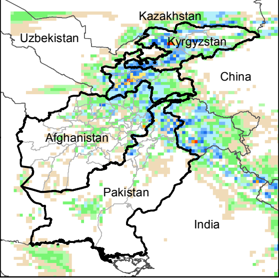
Daily Precip. Forecast for 14 Mar., 2016
