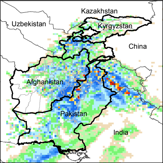
Daily Precip. Forecast for 11 Mar., 2016
