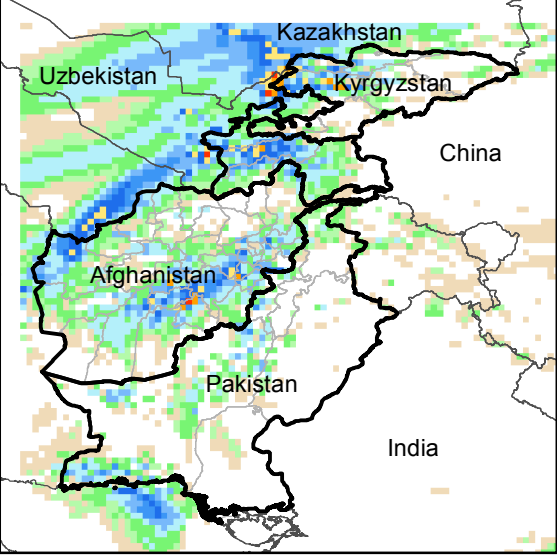
Daily Precip. Forecast for 15 Mar., 2016
