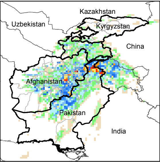
Daily Precip. Forecast for 25 Mar., 2016
