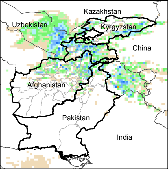
Daily Precip. Forecast for 14 Apr., 2016
