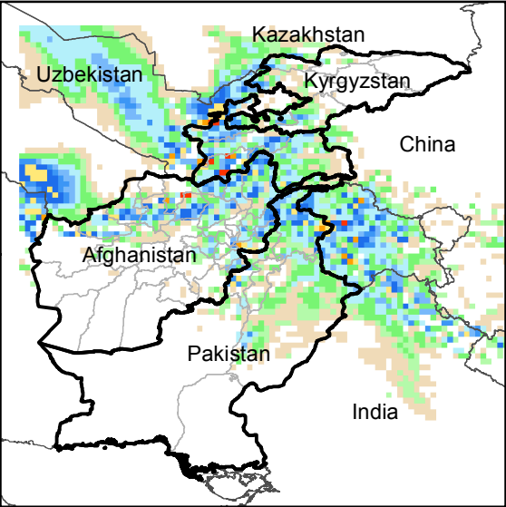
Daily Precip. Forecast for 20 Apr., 2016
