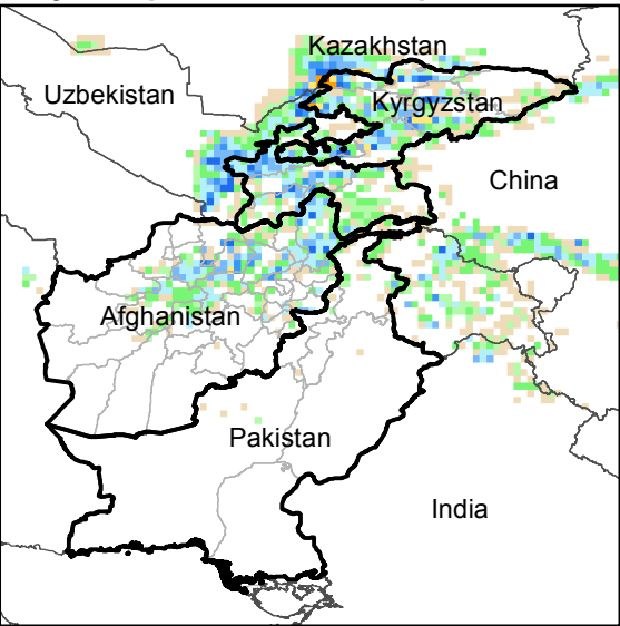
Daily Precip. Forecast for 23 Apr., 2016
