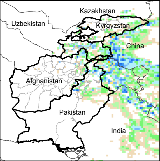
Daily Precip. Forecast for 24 May., 2016
