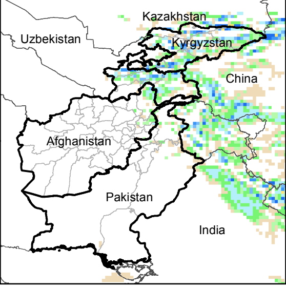
Daily Precip. Forecast for 28 May., 2016
