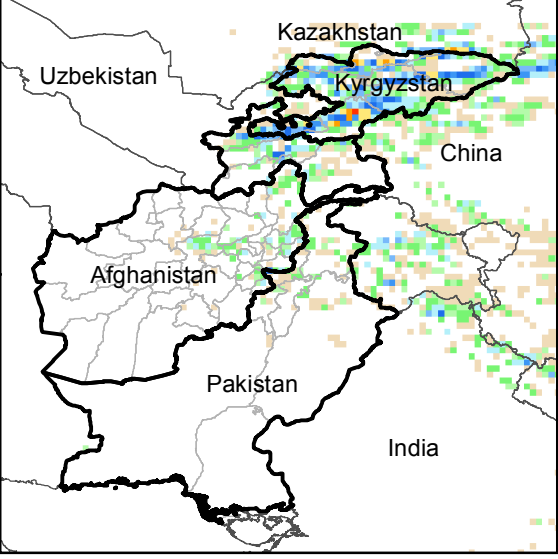
Daily Precip. Forecast for 27 May., 2016
