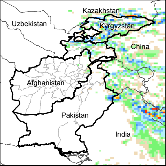
Daily Precip. Forecast for 29 May., 2016
