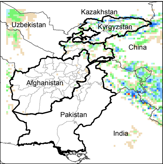
Daily Precip. Forecast for 11 Jun., 2016
