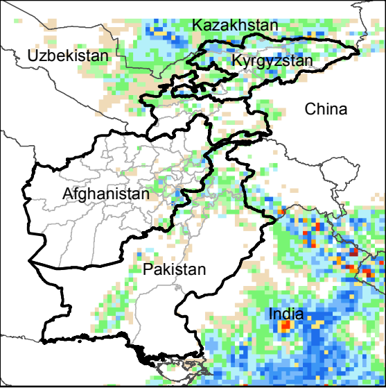
Daily Precip. Forecast for 27 Jun., 2016
