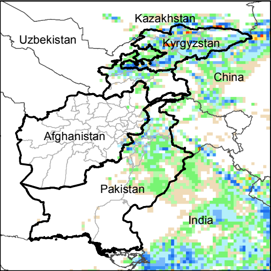
Daily Precip. Forecast for 22 Jun., 2016
