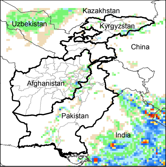
Daily Precip. Forecast for 26 Jun., 2016
