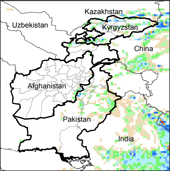
Daily Precip. Forecast for 23 Jun., 2016
