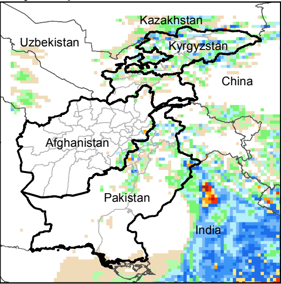
Daily Precip. Forecast for 4 Jul., 2016
