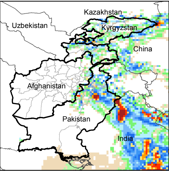
Daily Precip. Forecast for 6 Jul., 2016
