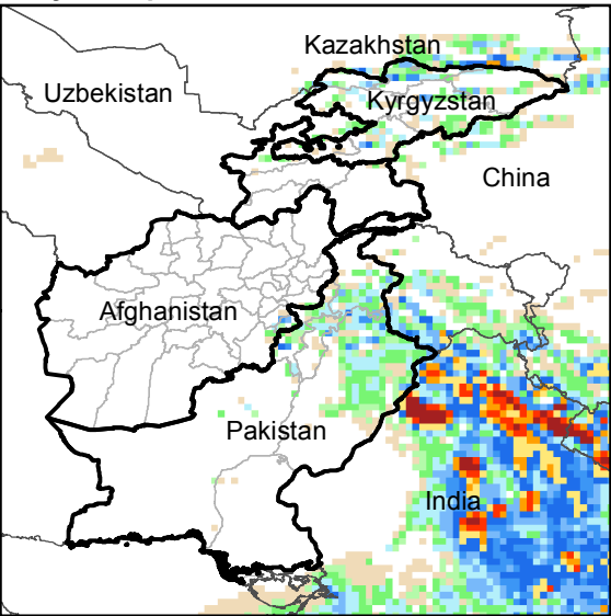
Daily Precip. Forecast for 5 Jul., 2016
