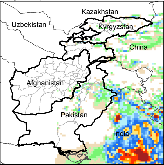
Daily Precip. Forecast for 10 Jul., 2016
