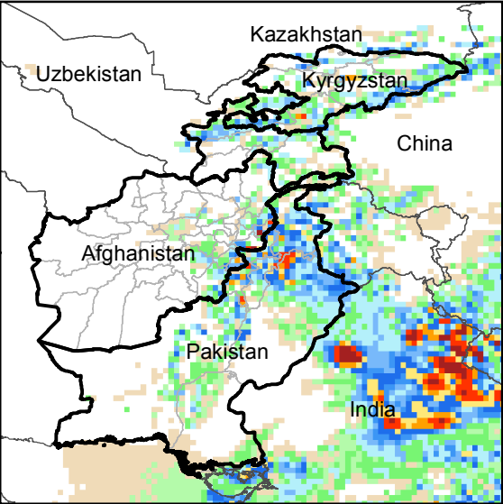
Daily Precip. Forecast for 20 Jul., 2016
