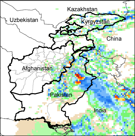
Daily Precip. Forecast for 21 Jul., 2016
