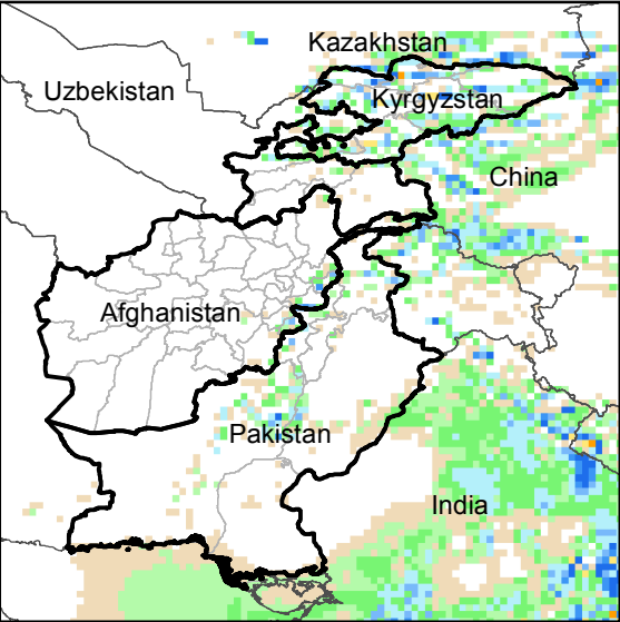
Daily Precip. Forecast for 22 Jul., 2016
