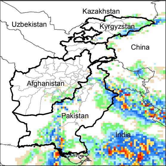
Daily Precip. Forecast for 6 Aug., 2016
