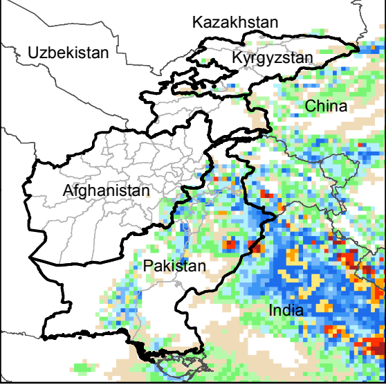
Daily Precip. Forecast for 8 Aug., 2016
