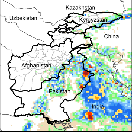
Daily Precip. Forecast for 7 Aug., 2016
