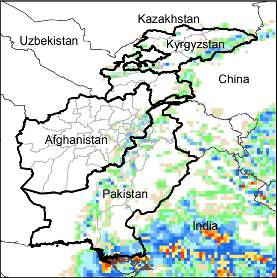
Daily Precip. Forecast for 4 Aug., 2016
