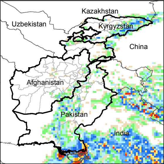
Daily Precip. Forecast for 5 Aug., 2016
