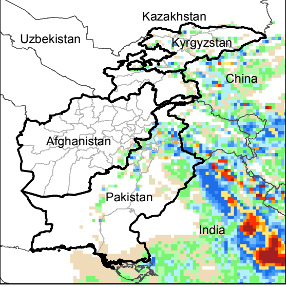
Daily Precip. Forecast for 9 Aug., 2016
