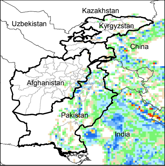
Daily Precip. Forecast for 29 Aug., 2016
