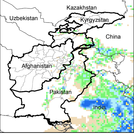
Daily Precip. Forecast for 1 Sep., 2016
