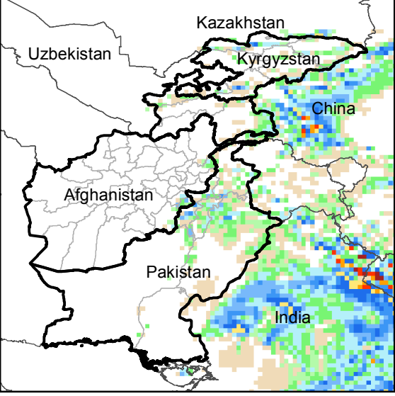
Daily Precip. Forecast for 30 Aug., 2016
