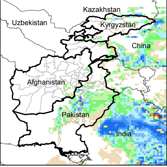
Daily Precip. Forecast for 31 Aug., 2016
