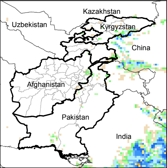
Daily Precip. Forecast for 15 Sep., 2016
