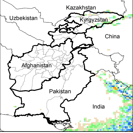
Daily Precip. Forecast for 20 Sep., 2016
