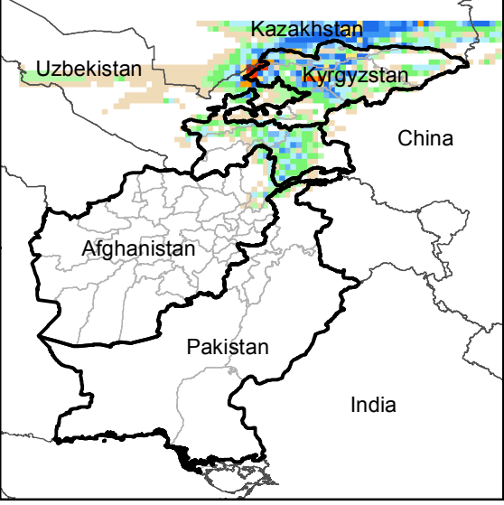
Daily Precip. Forecast for 16 Nov., 2016
