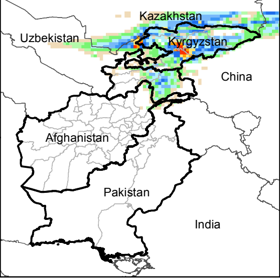
Daily Precip. Forecast for 17 Nov., 2016
