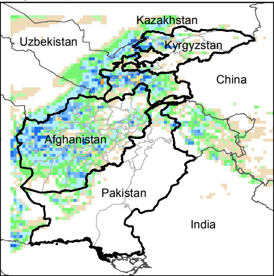
Daily Precip. Forecast for 25 Jan., 2017
