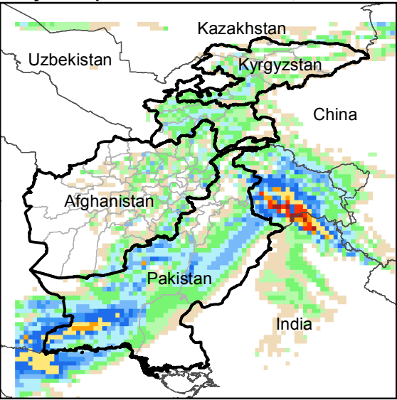
Daily Precip. Forecast for 24 Jan., 2017
