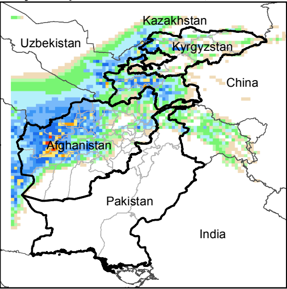
Daily Precip. Forecast for 2 Feb., 2017
