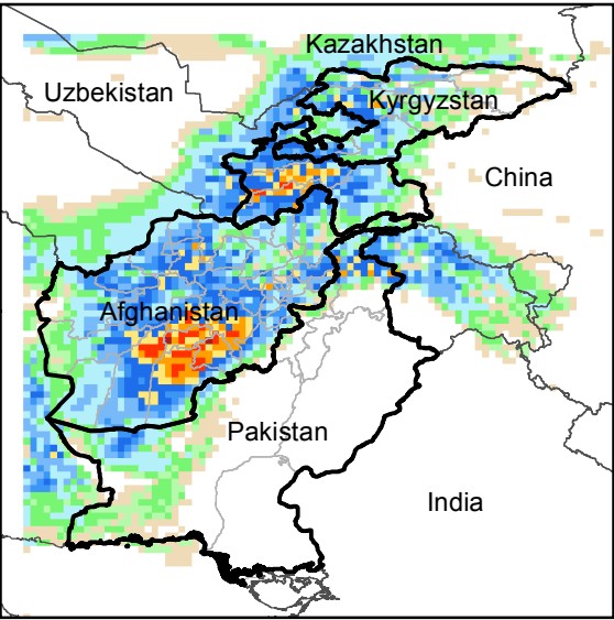
Daily Precip. Forecast for 3 Feb., 2017
