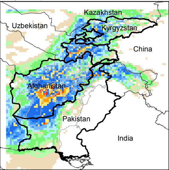
Daily Precip. Forecast for 6 Feb., 2017
