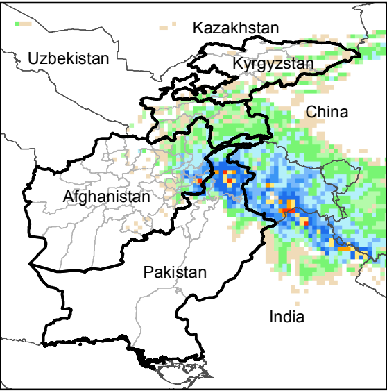
Daily Precip. Forecast for 5 Feb., 2017
