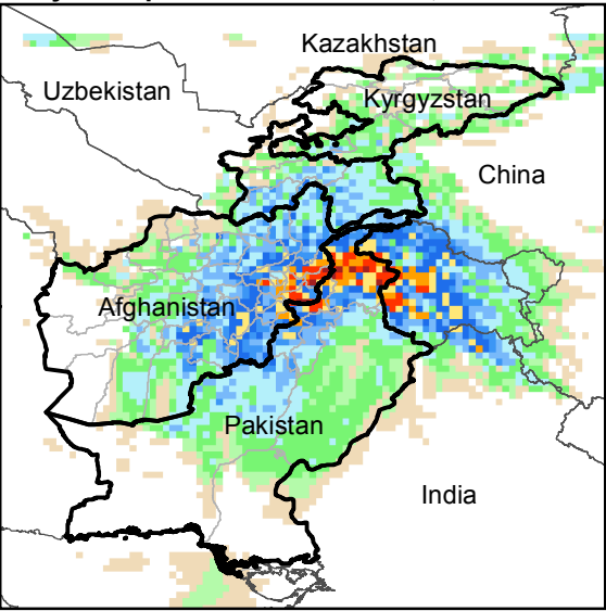
Daily Precip. Forecast for 4 Feb., 2017
